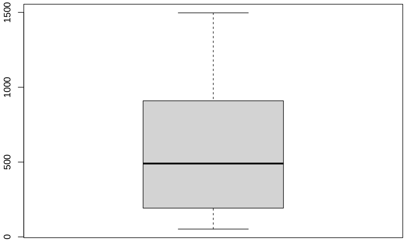
Boxplot – Precipitation
