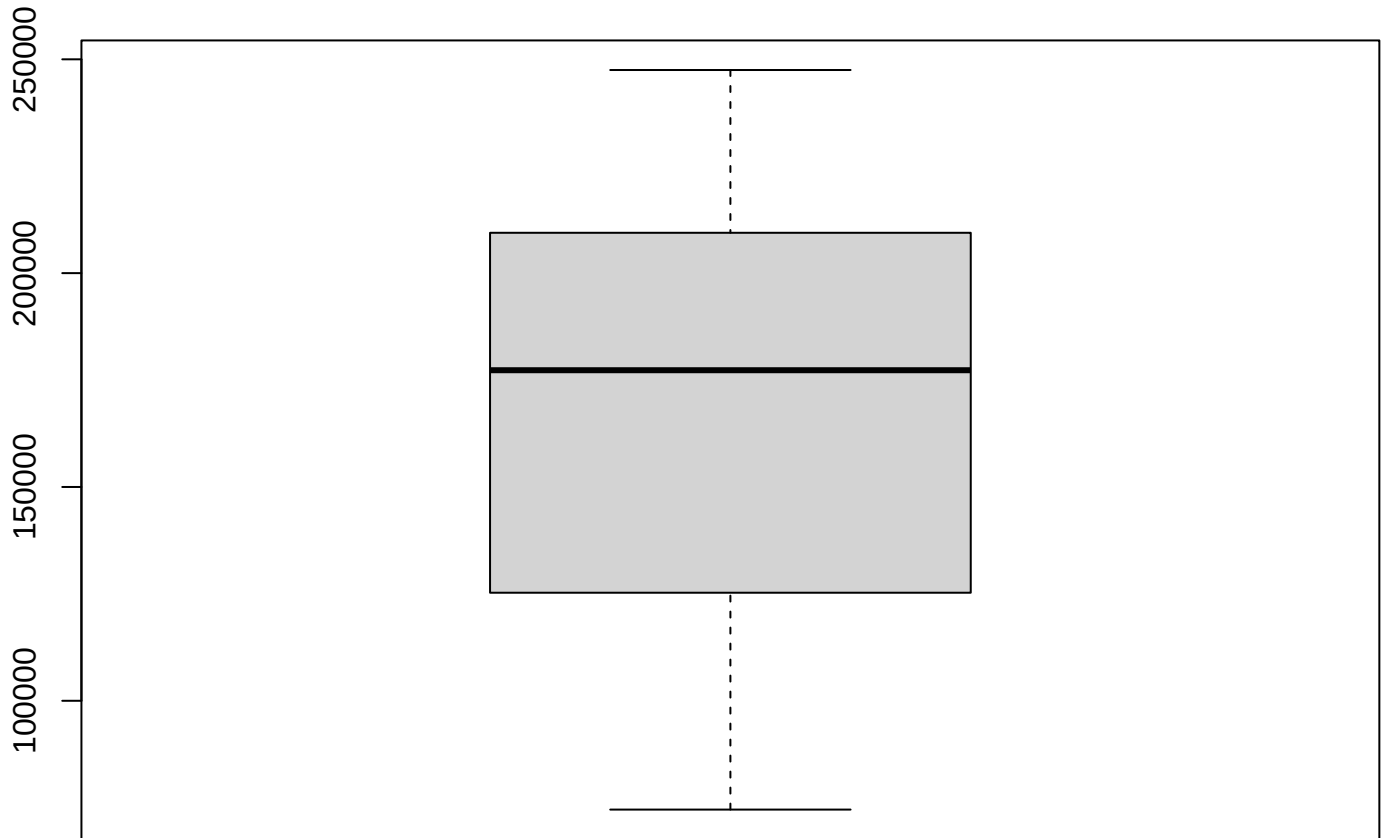
Boxplot – Discharge
