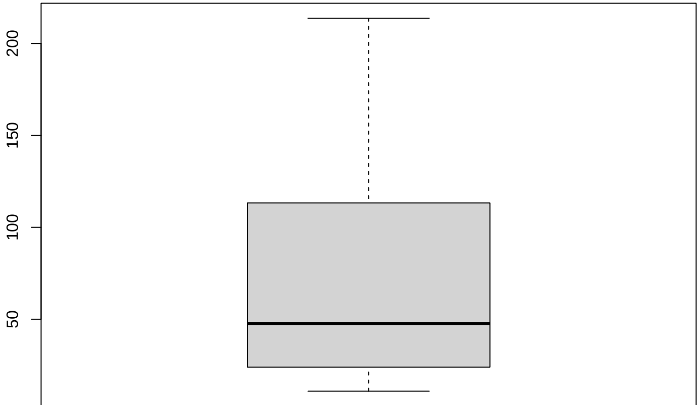
Boxplot – TSS
